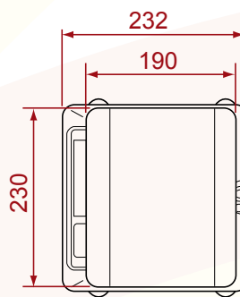
PLAN VIEW
